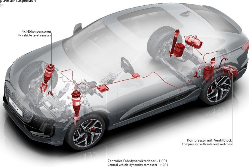
adaptive air suspension 10/24
